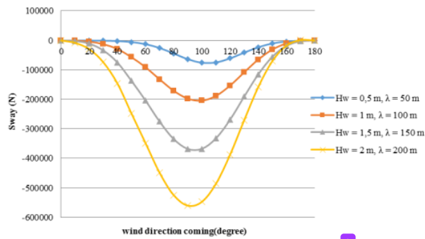
Figure 11. Sway force at various angles of wind for a wind speed of 0 m/s
