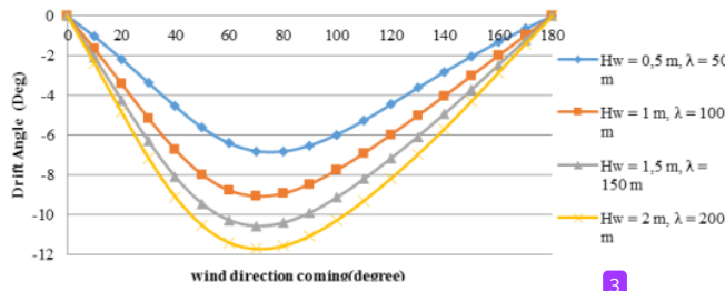
Figure 13. Drift angle at various incident wind angles for a wind speed of 10 m/s
